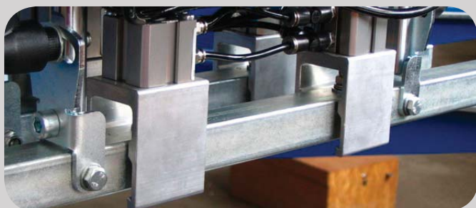
Squeegee & Floodbar Air Clamps
